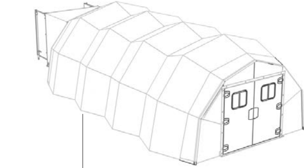
Arch modules are interoperable and allow shelters to increase in size or add functions with added arches
